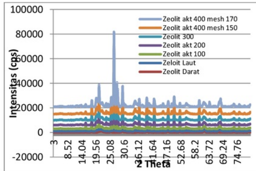
Figure 4. Characterized by X - Ray Difraction type Rigaku Miniflex II
