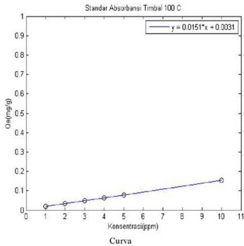
Figure 5. Curva standar Of Lead (Pb)
